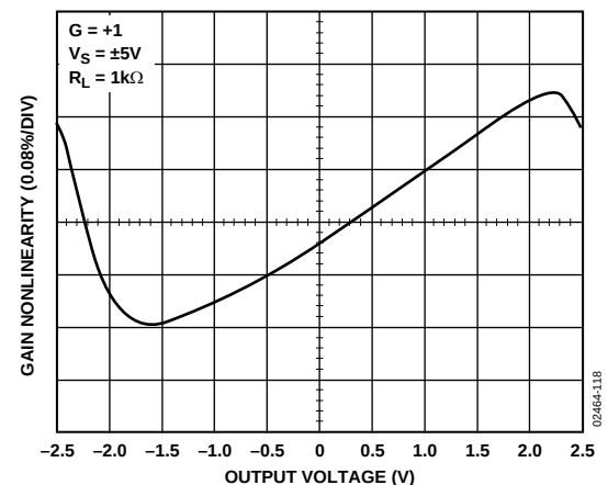
Figure 117. AD8130 Gain Nonlinearity, V_{OUT} = 5V p-p
