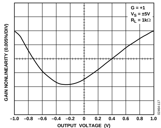
Figure 116. AD8130 Gain Nonlinearity, V_{OUT} = 2V p-p
