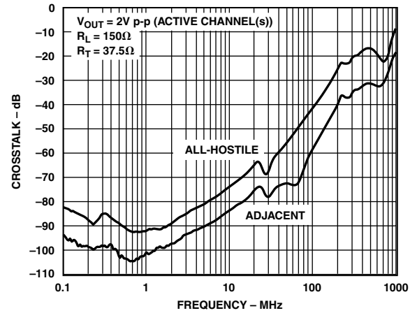
TPC 9. AD8075 Crosstalk vs. Frequency (All Hostile and Adjacent R_L = 150\text{ }\Omega )
