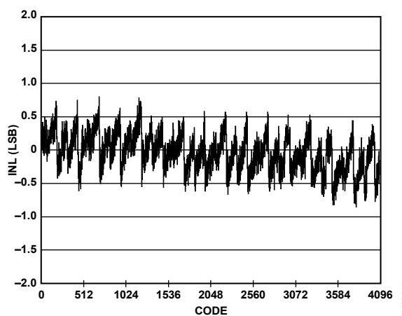
Figure 14. ADC INL
