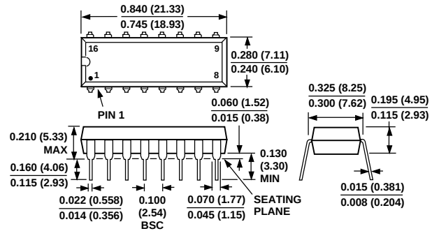
Plastic DIP (N-16)
