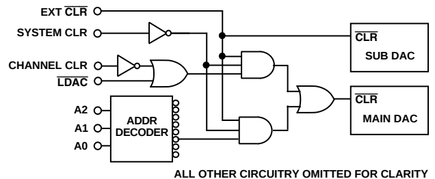
Figure 20. \overline{\text{CLR}} Functions for Main and Sub DACs
