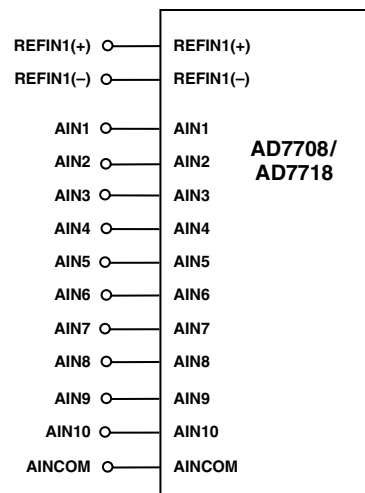
Figure 24. Analog Input and Reference Options with CHCON = 1
