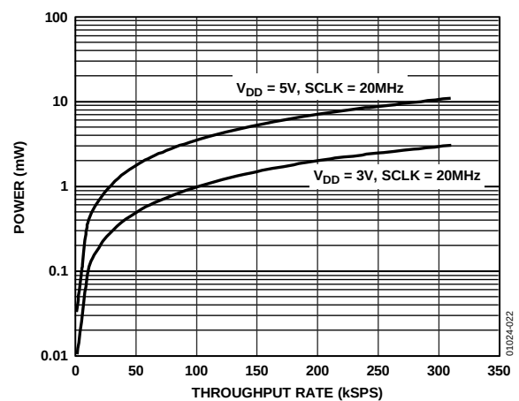
Figure 22. Power vs. Throughput Rate
