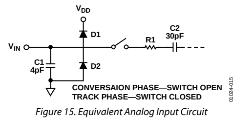
Figure 15. Equivalent Analog Input Circuit
