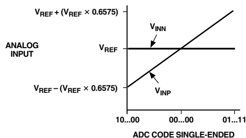
Figure 8. ADC Transfer Function
