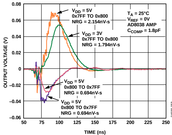
Figure 25. Midscale Transition, V_{REF} = 0\text{V}
