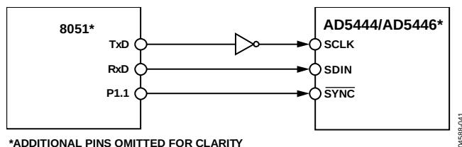
Figure 49. 80C51/80L51 to AD5444/AD5446 Interface
