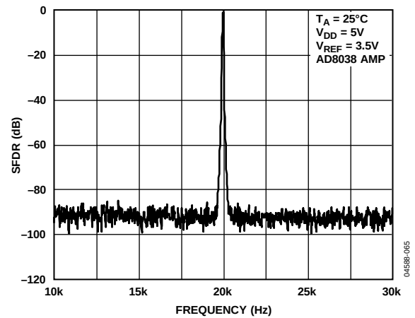
Figure 32. Narrow-Band SFDR, f_{OUT} = 20 kHz, Clock = 1 MHz
