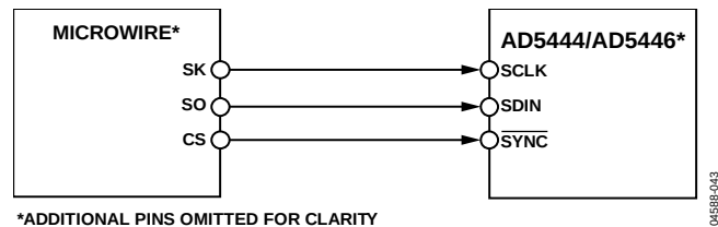
Figure 51. MICROWIRE to AD5444/AD5446 Interface
