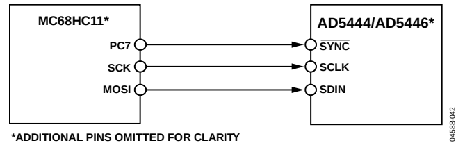
Figure 50. MC68HC11 to AD5444/AD5446 Interface
