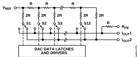
Figure 37. Simplified Ladder
