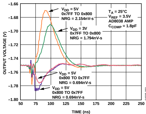
Figure 26. Midscale Transition, V_{REF} = 3.5\text{V}
