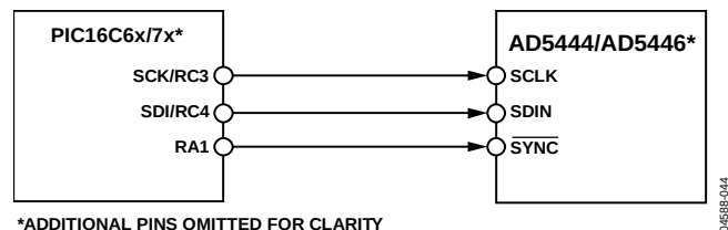
Figure 52. PIC16C6x/7x to AD5444/AD5446 Interface
