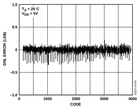
Figure 19. AD5348 Typical DNL Plot
