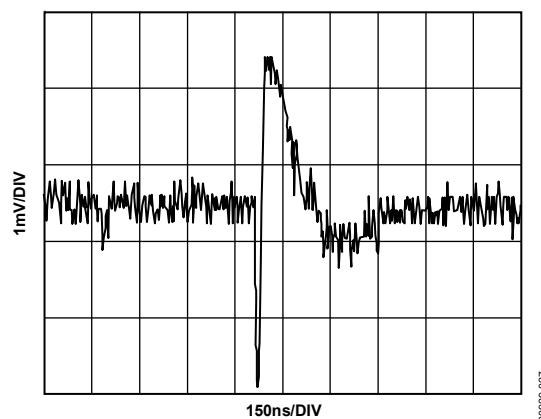
Figure 27. DAC-to-DAC Crosstalk
