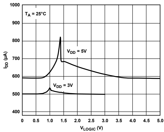
Figure 19. Supply Current vs. Logic Input Voltage
