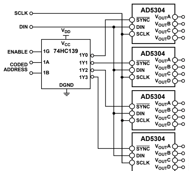
Figure 43. Decoding Multiple AD5304 Devices in a System
