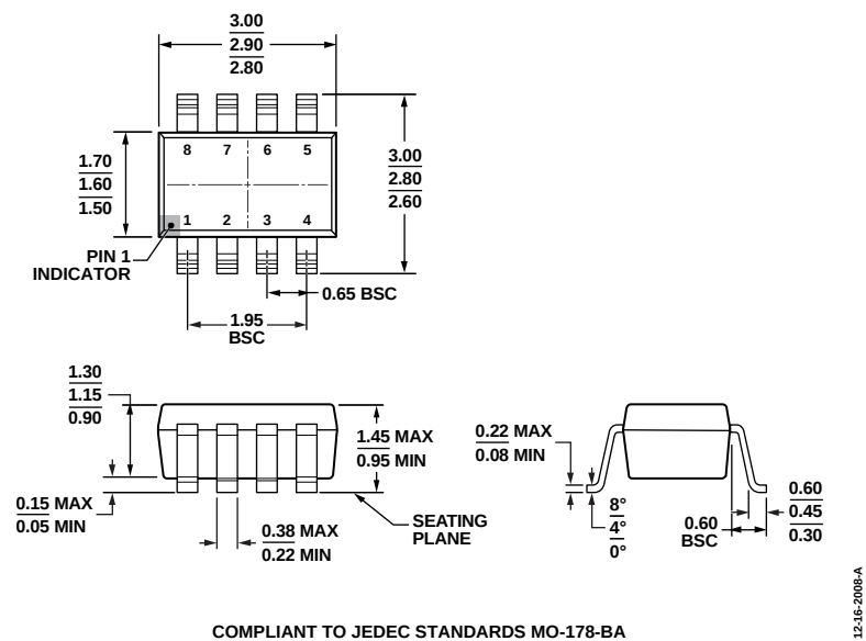
Figure 43. 8-Lead Small Outline Transistor Package [SOT-23] (RJ-8) Dimensions shown in millimeters
