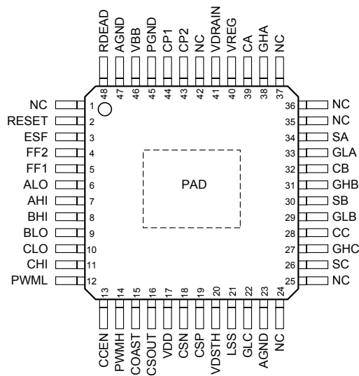
Pinout Diagram
