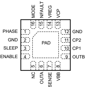
EU-16 Pinout Diagram
