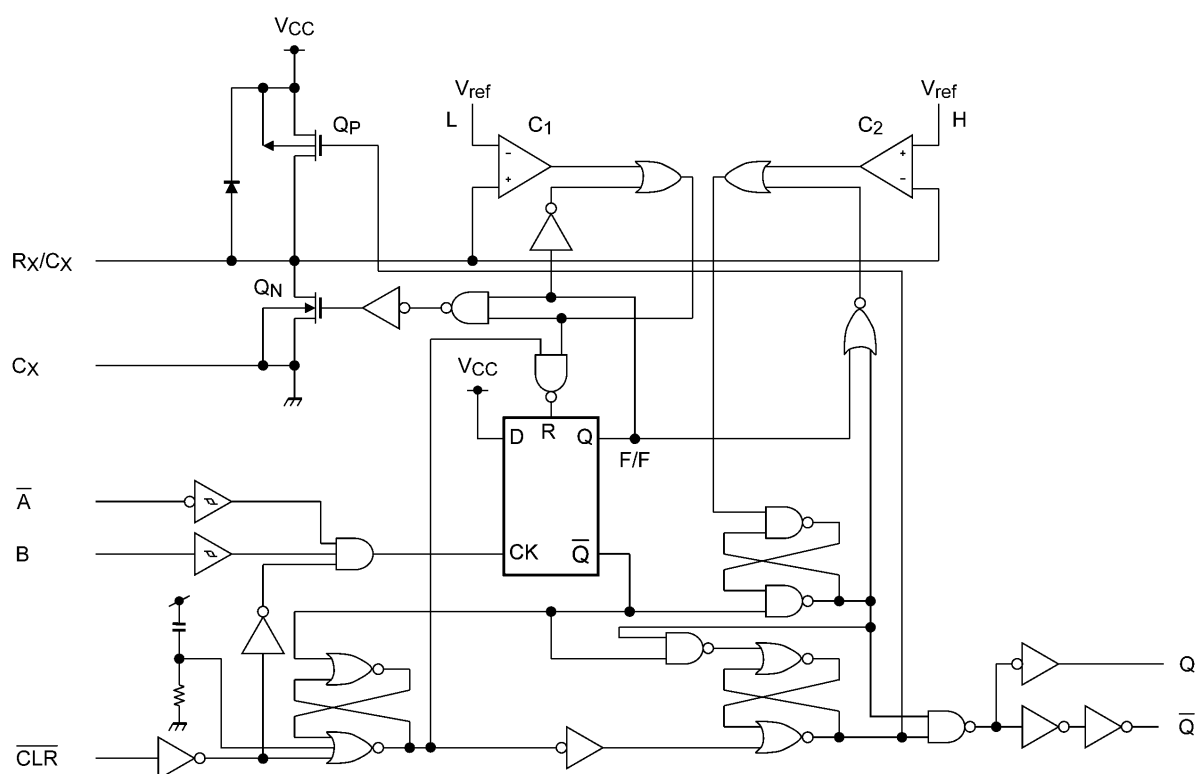
Fig. 10.1 74VHC123AFT
