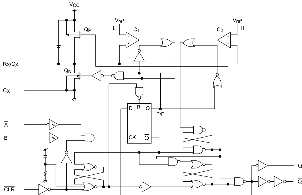
Fig. 10.2 74VHC221AFT
