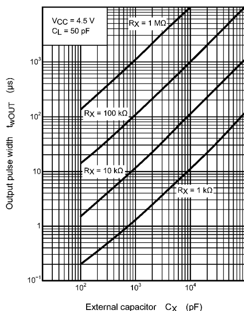
Fig. 16.1 t_{OUT} - C_X (typ.)
