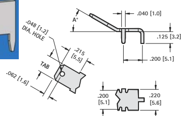
.110 (2.8) & .187 (4.8) TAB
