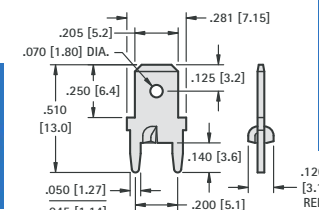
.205 (5.2) TAB
