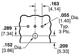
3 Circuit, In-Line
