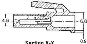
Section X-X
