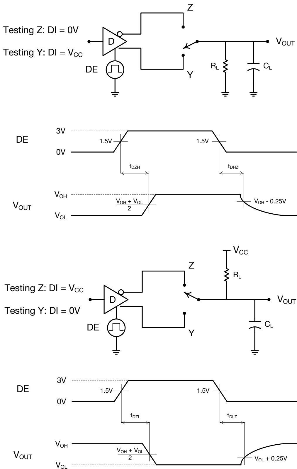
Figure 7: Driver Enable and Disable Timing Test Circuits and Timing Diagrams
