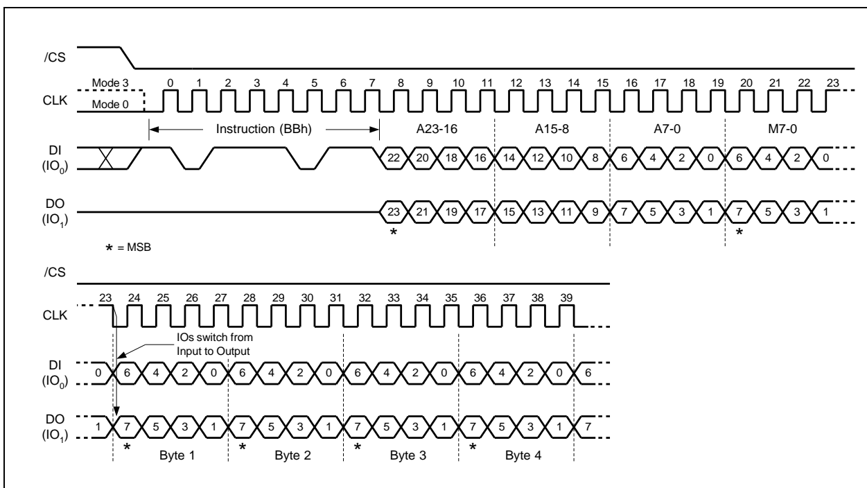
Figure 22a. Fast Read Dual I/O Instruction (Initial instruction or previous M5-4 \neq 10, SPI Mode only)
