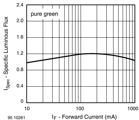
Figure 27. Specific Luminous Intensity vs. Forward Current
