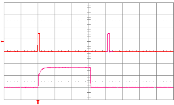
Figure 16. Load current (top trace, 20 A/div., 50 ms/div.) into a 10 m \Omega short circuit during restart, at V_{in} = 48V . Bottom trace (10 A/div., 2 ms/div.) is an expansion of the on-time portion of the top trace.
