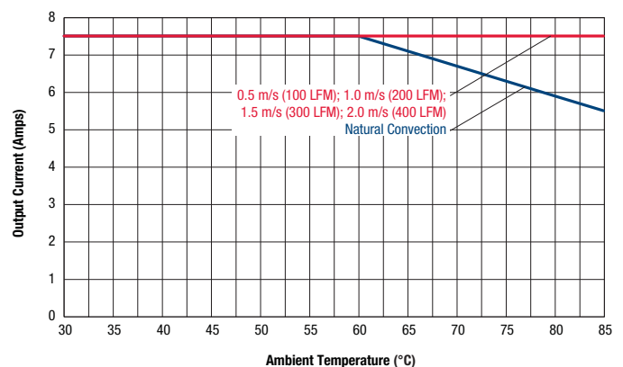
Maximum Current Temperature Derating at sea level Vin = 48 (air flow from J1 to J3 on PCB)
