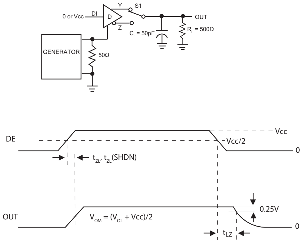
Figure 6. Driver Enable and Disable Times Test Circuit and Timing Diagram
