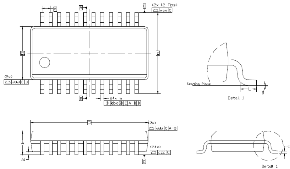
Figure 5. 24-Pin SSOP
