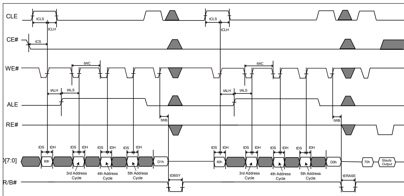
Figure 37. AC Waveforms for Two-plane Erase (ONFI)
