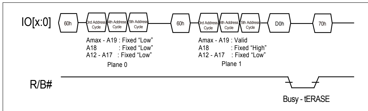
Figure 40. AC waveforms for Two-plane Erase (Traditional)
