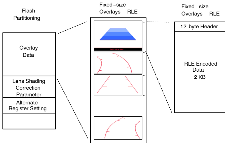
Figure 36. Memory Partitioning
