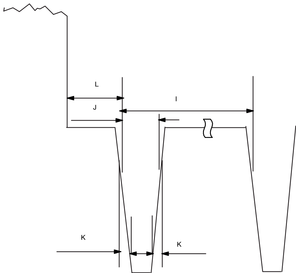
Figure 62. Equivalent Pulse
