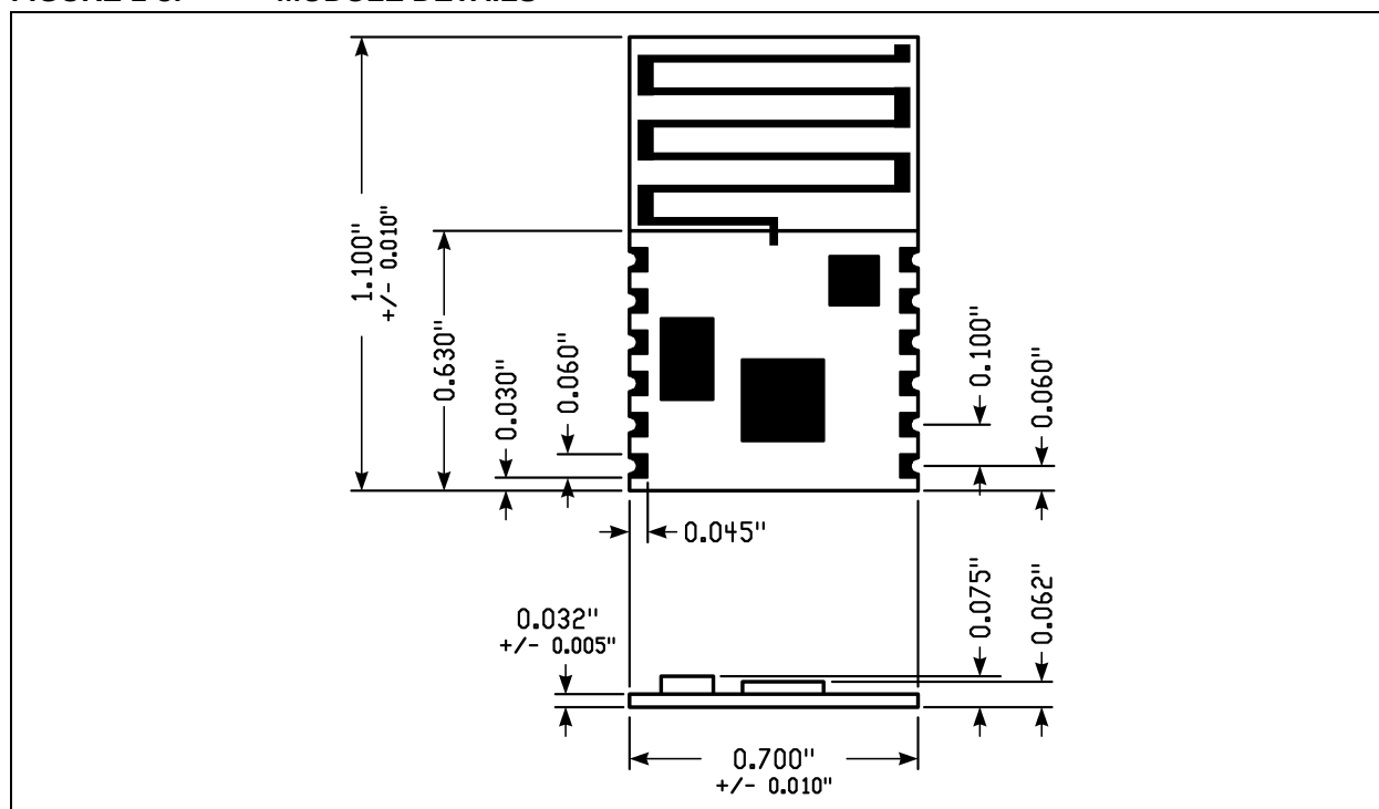
FIGURE 1-3: MODULE DETAILS
