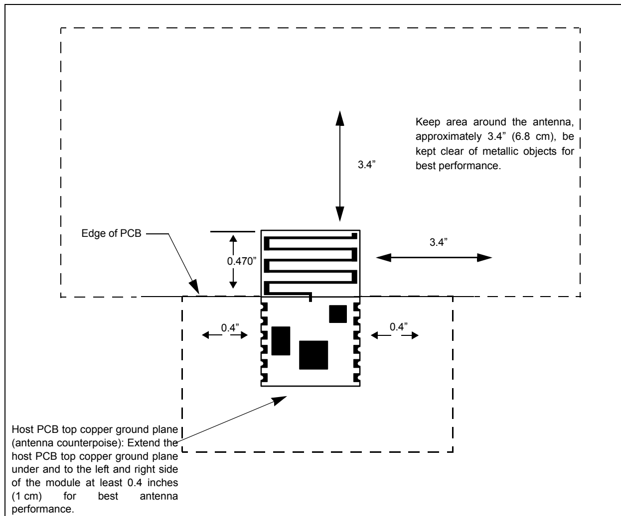
FIGURE 1-5: MOUNTING DETAILS
