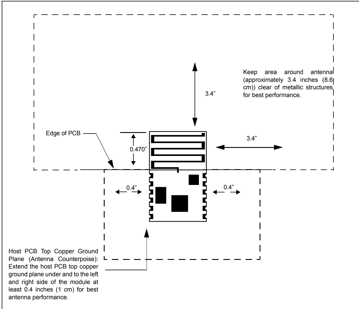
FIGURE 1-5: MOUNTING DETAILS
