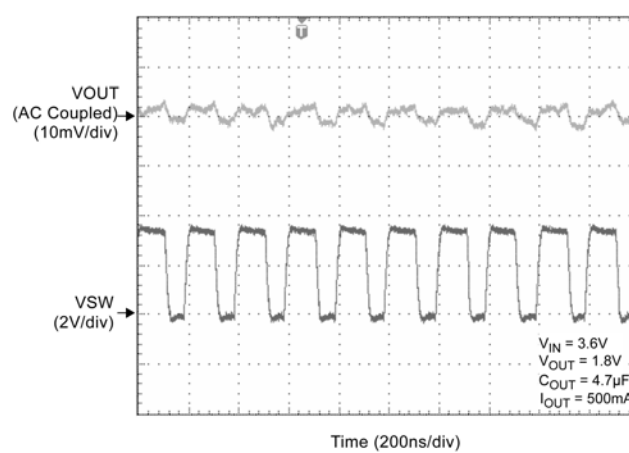
Switching Waveform
