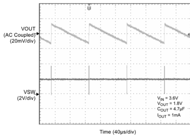
Switching Waveform
