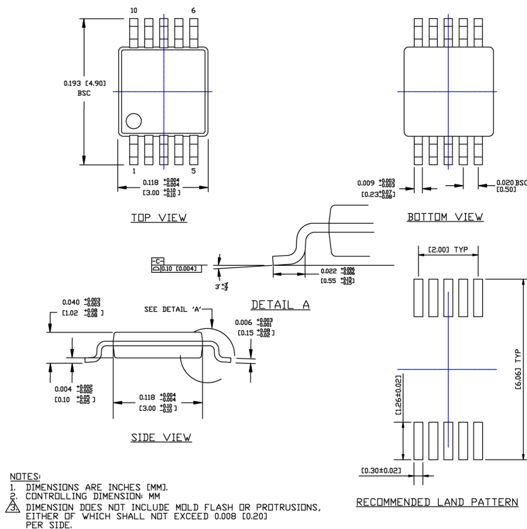
10-Pin MSOP (MM)
