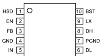
10-Pin MSOP (MM)
