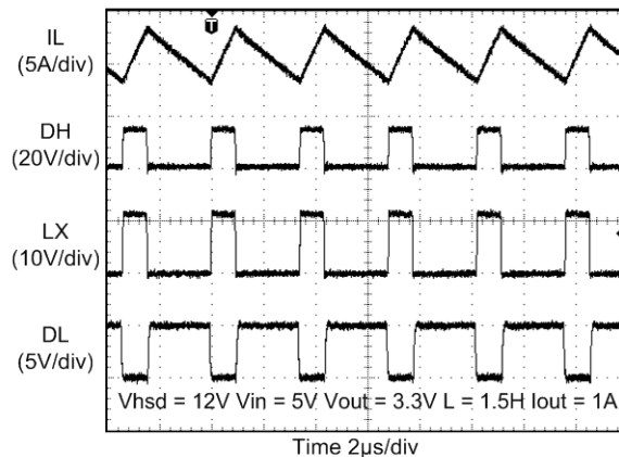
MIC2164 Switching Waveforms (Light Load)
