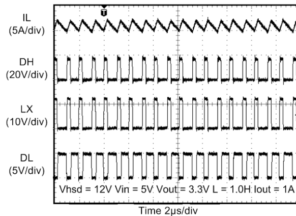
MIC2164-3 Switching Waveforms (Light Load)
