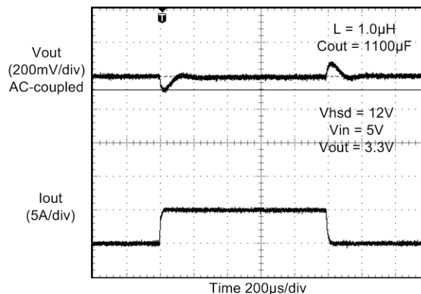
MIC2164-2 Load Transient
