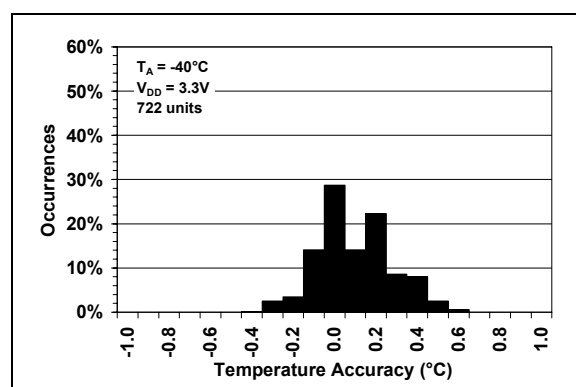
FIGURE 2-6: Temperature Accuracy Histogram, T_A = -40^{\circ}C .
