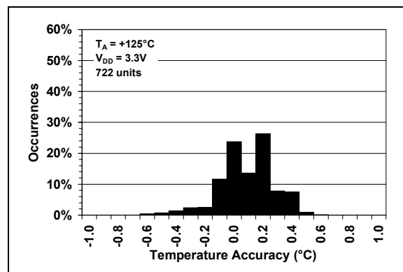
FIGURE 2-5: Temperature Accuracy Histogram, T_A = +125^{\circ}C .
