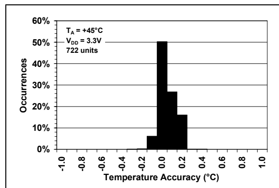
FIGURE 2-4: Temperature Accuracy Histogram, T_A = +45^{\circ}C .
