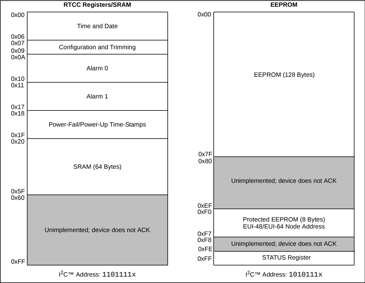
FIGURE 5-1: MEMORY MAP
