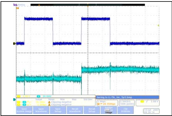
FIGURE 2-16: 5 k \Omega – Low-Voltage Increment Wiper Settling Time ( V_{DD} = 5.5V ) (1 \mu s/Div ).
