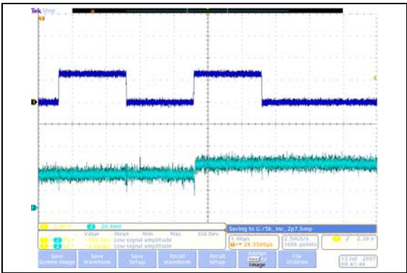
FIGURE 2-17: 5 k \Omega – Low-Voltage Increment Wiper Settling Time ( V_{DD} = 2.7V ) (1 \mu s/Div ).
