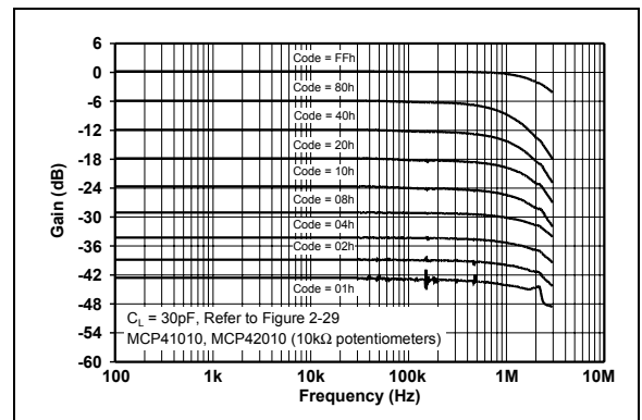
FIGURE 2-18: Gain vs. Frequency for 10 k \Omega Potentiometer.
