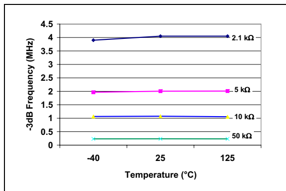
FIGURE 2-48: -3 dB Bandwidth vs. Temperature.
