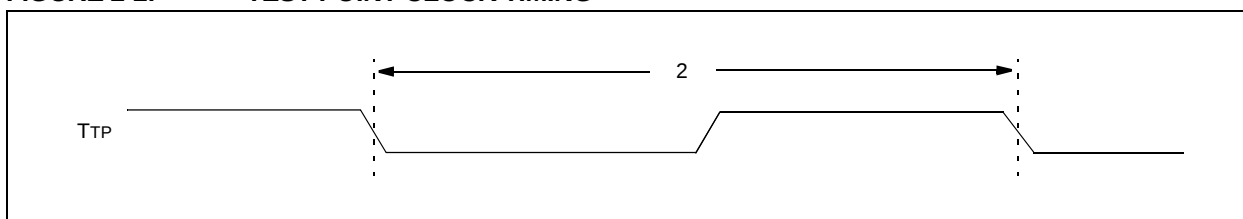
FIGURE 2-2: TEST POINT CLOCK TIMING
