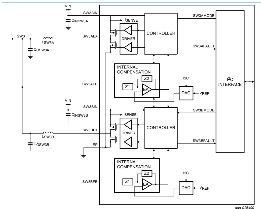
Figure 21. SW3A/B dual phase block diagram
