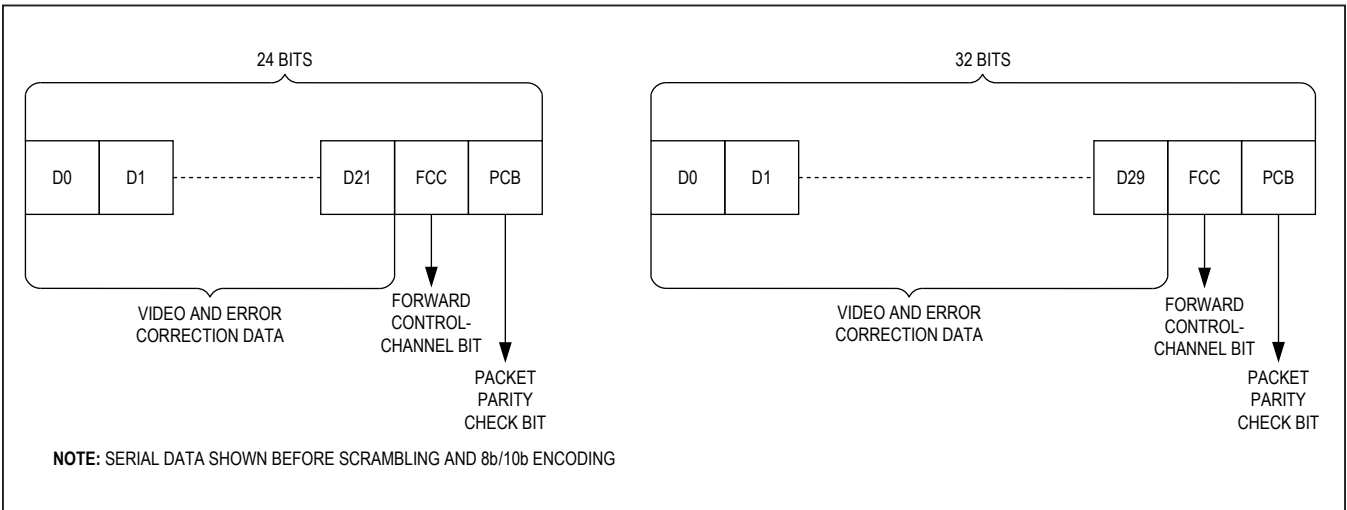
Figure 15. Serial-Data Format
