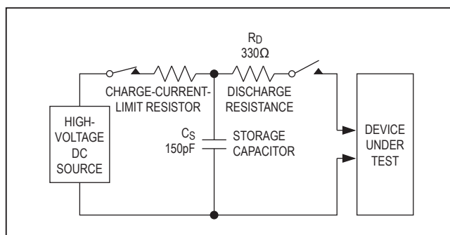
Figure 33. IEC 61000-4-2 Contact Discharge ESD Test Circuit
