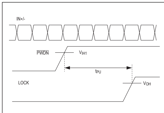
Figure 10. Power-Up Delay
