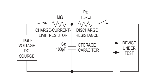
Figure 32. Human Body Model ESD Test Circuit
