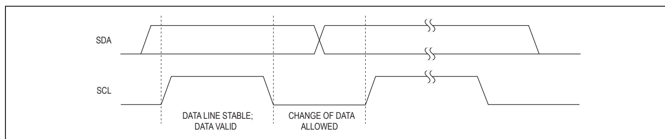
Figure 23. Bit Transfer
