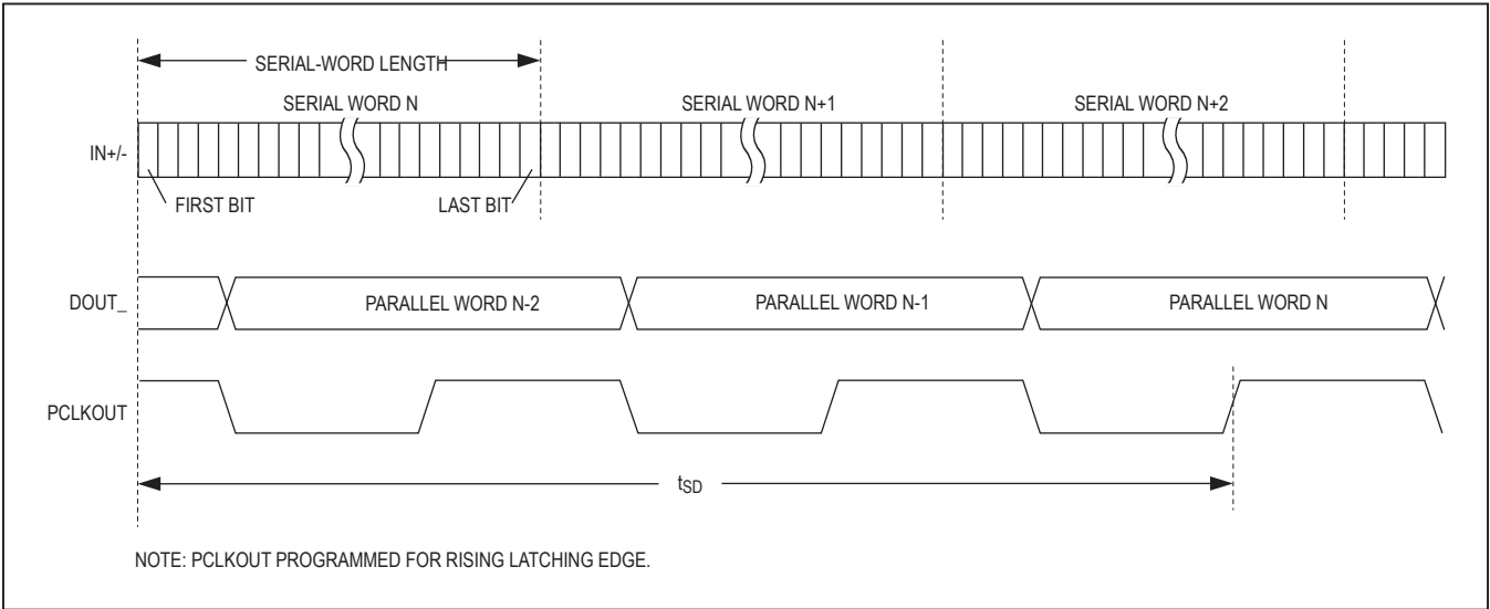
Figure 7. Deserializer Delay
