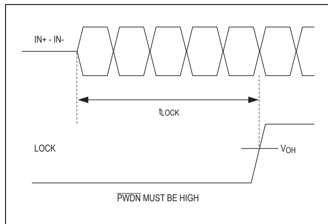
Figure 9. Lock Time
