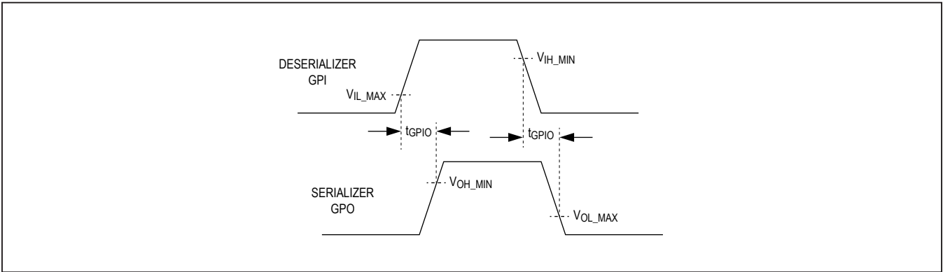
Figure 8. GPI-to-GPO Delay
