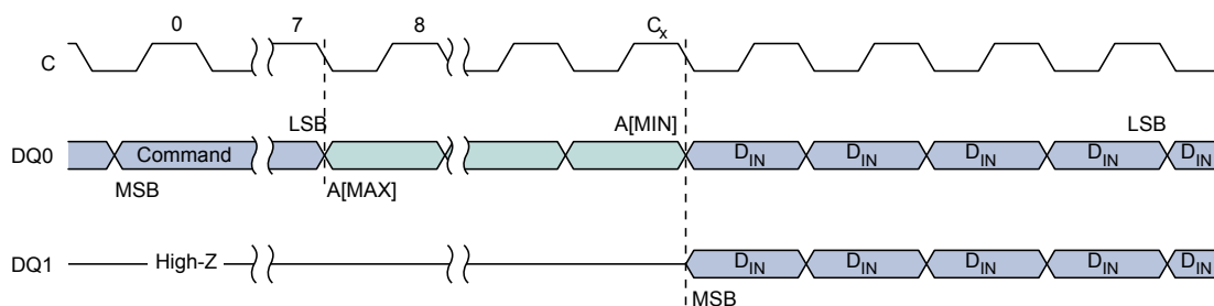
Figure 20: DUAL INPUT FAST PROGRAM Command Sequence
