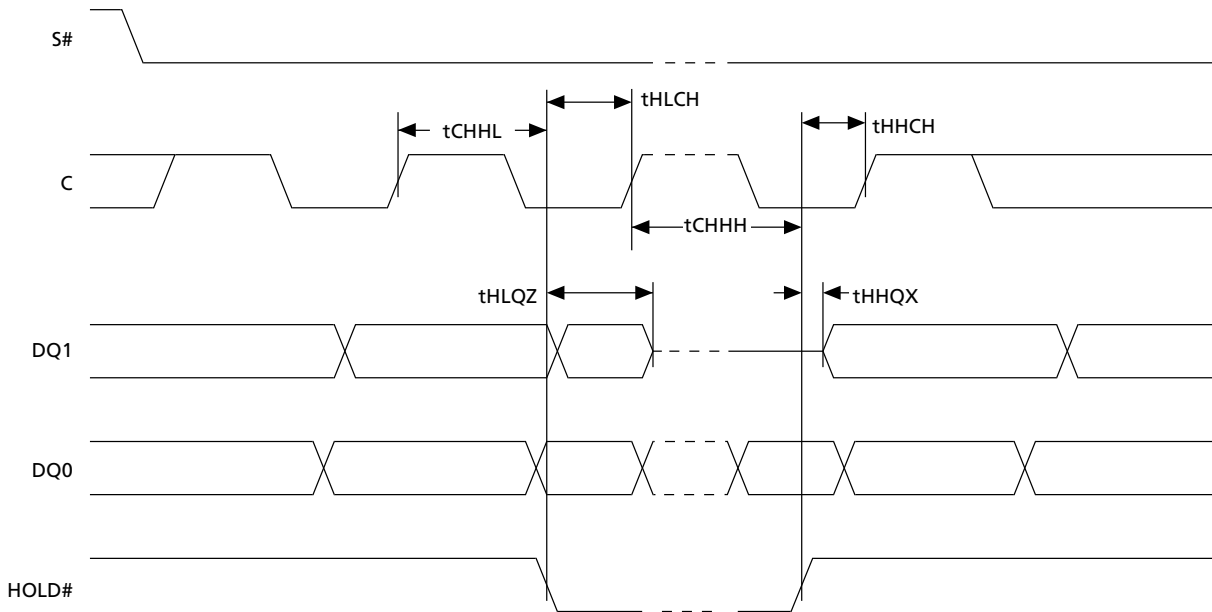
Figure 33: Hold Timing
