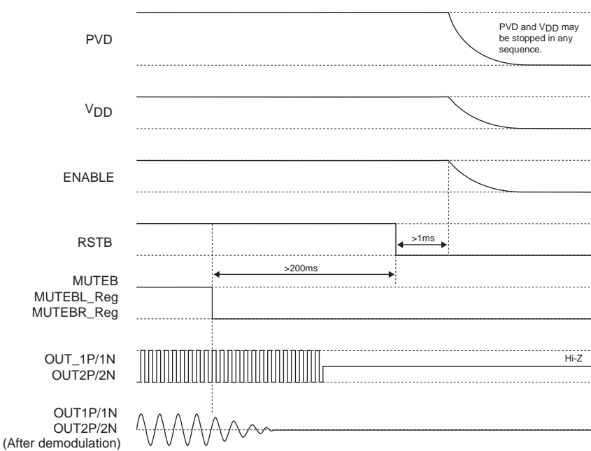
Figure 3.2 Stop sequence
