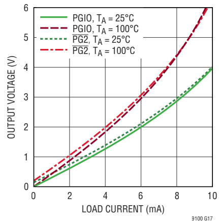
PG2, PG10 Output Low Voltage vs Load Current
