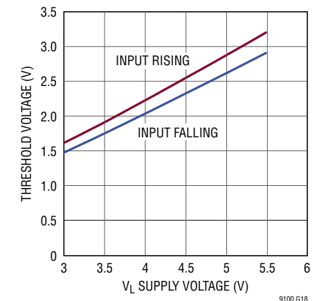
Logic Input Threshold vs V_L Supply Voltage
