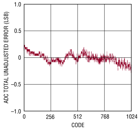
ADC Total Unadjusted Error vs Code (ADIN Pin)
