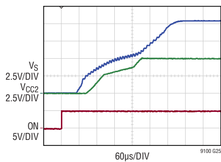
Power-On Sequence
