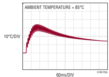
Figure 20(c). Q1 Junction Temperature
