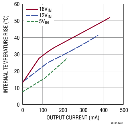
Internal Temperature Rise vs Output Current, 15V OUT SEPIC
