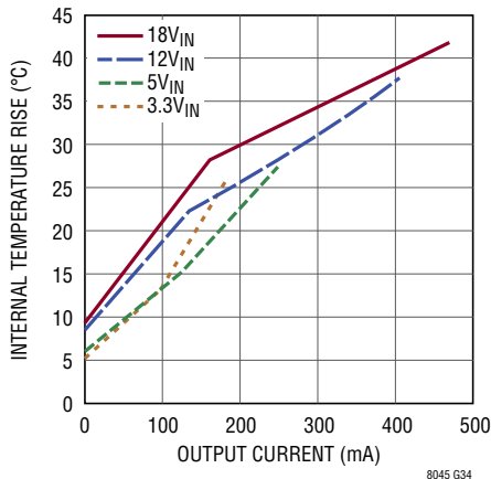
Internal Temperature Rise vs Output Current, 12V OUT SEPIC
