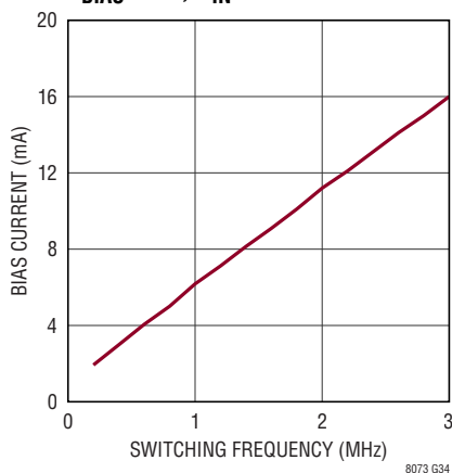
I_{BIAS} vs Switching Frequency V_{BIAS} = 5V , V_{IN} = 24V
