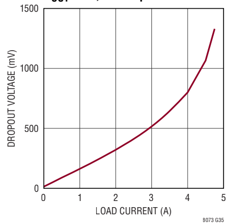
Dropout Voltage vs Load Current V_{OUT} = 5V , BIAS Open
