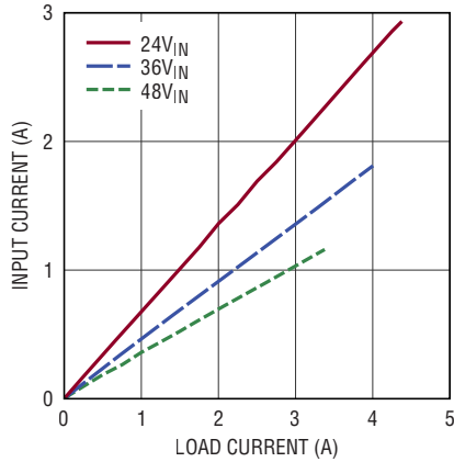
Input vs Load Current V_{OUT} = 15V
