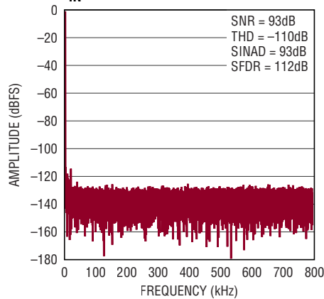
32k Point FFT f_{\text{SAMPL}} = 1.6\text{MSPS} , f_{\text{IN}} = 1\text{kHz}
