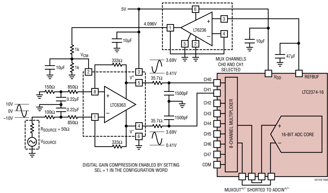
LTC6363 Configured to Accept a ±10V Input Signal Using a Single 5V Supply with Digital Gain Compression Enabled on the LTC2374-16
