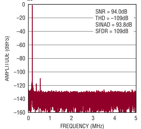
32k Point FFT f_{\text{SAMPL}} = 10\text{Mps} , f_{\text{IN}} = 200\text{kHz}
