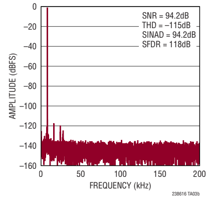
128k Point FFT, f_{\text{SAMPL}} = 10\text{Mps} , f_{\text{IN}} = 8\text{kHz} (Zoomed View)
