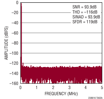
32k Point FFT, f_{\text{SAMPL}} = 10\text{Mps} , f_{\text{IN}} = 50\text{kHz}
