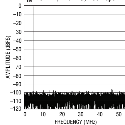
LTC2267-12: 8k Point FFT, f_{IN} = 5\text{MHz} , -1dBFS, 105Mps
