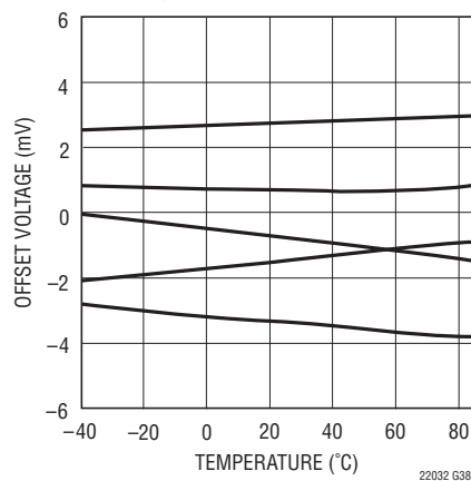
LTC2203: Offset Voltage vs Temperature, 5 Units
