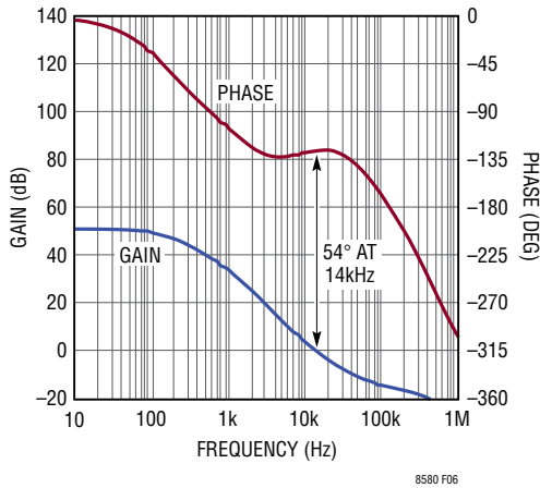
Figure 6. Bode Plot for Example Boost Converter
