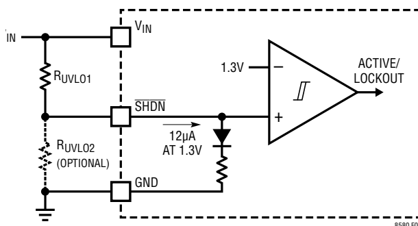
Figure 8. Configurable UVLO
