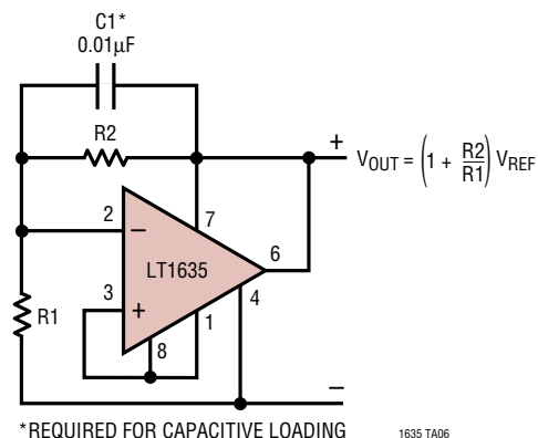
Shunt Regulator
