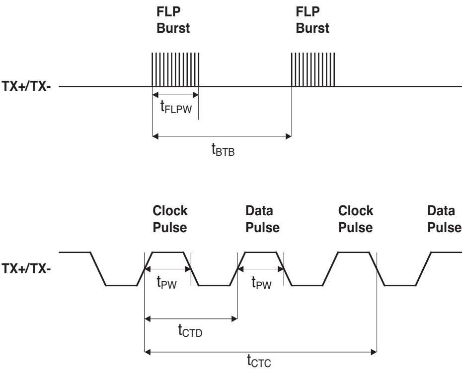
Figure 8. Auto-Negotiation/Fast Link Pulse Timing
