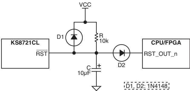
Figure 11. Recommended Reset Circuit.
