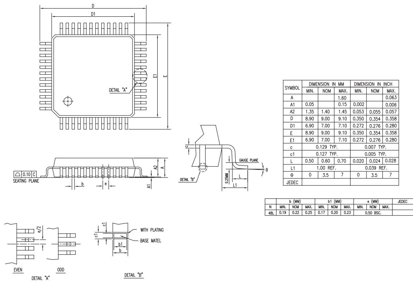
48-pin LQFP (LQ)
