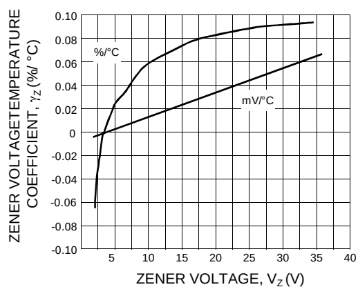
FIG.2 - TEMPERATURE COEFFICIENT vs. ZENER VOLTAGE
